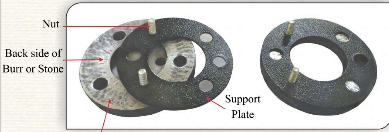
Stone / Burr Support Plate with Bolt-Nut Kit.
